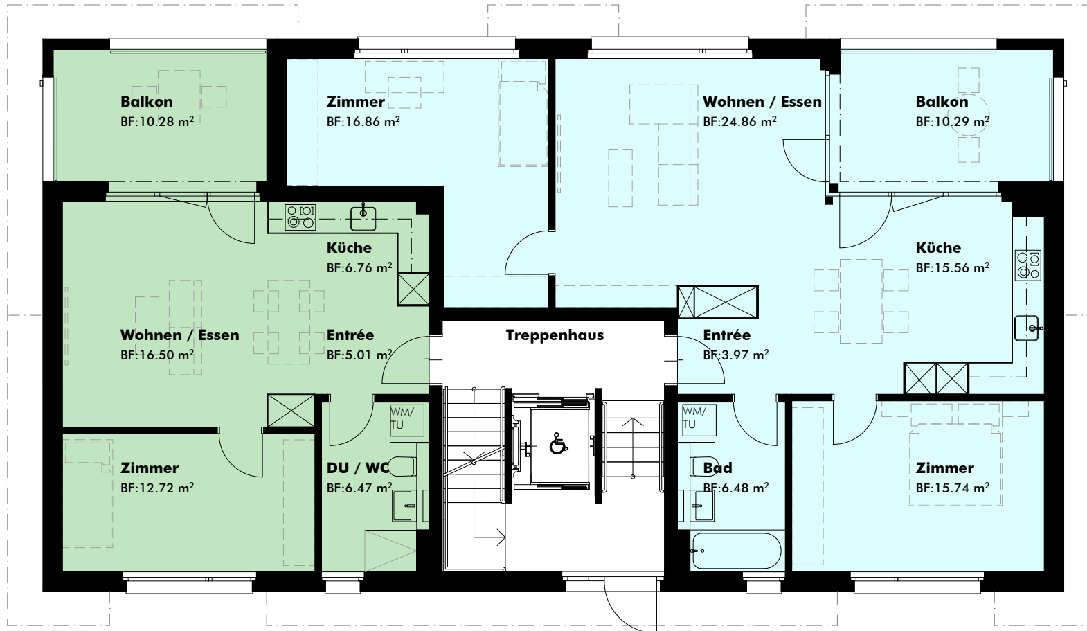
WHG 04-01-02 2 Zimmer
